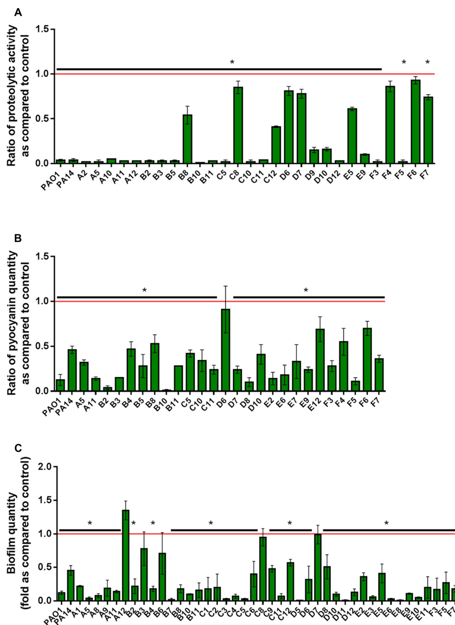
FIGURE 3 | Quenching of virulence factors using SsoPox. For each strain, bars represent the mean ratios of protease (A), pyocyanin (B) and biofilm (C) levels between the treated culture with 0.5 \text{ mg ml}^{-1} SsoPox versus the untreated culture of three experiments. Error bars represent the standard deviations of three replicated experiments. * p -values < 0.05 according to Student's t -test.
